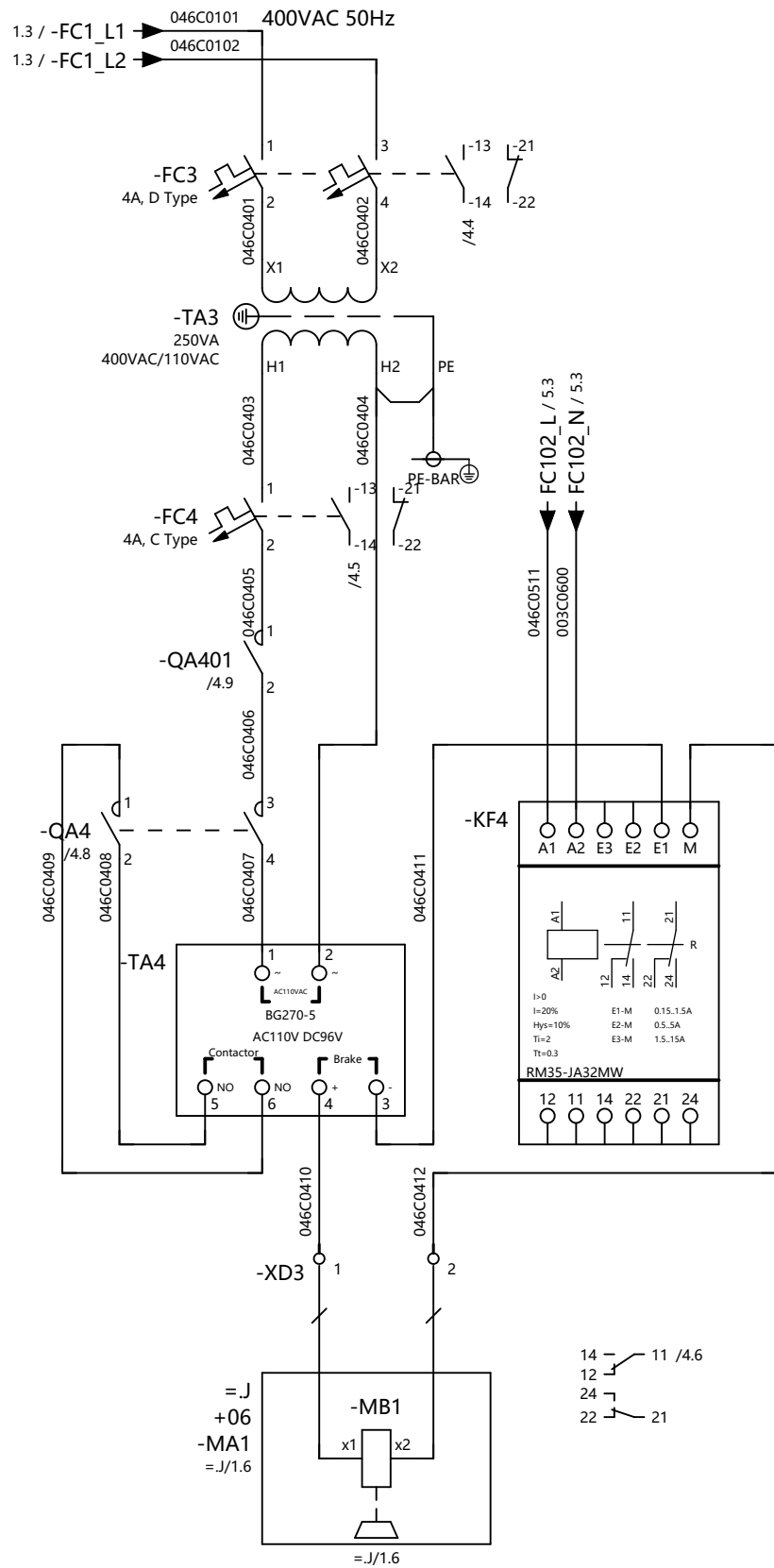
GANTRY CABLE REEL MOTOR BRAKE
