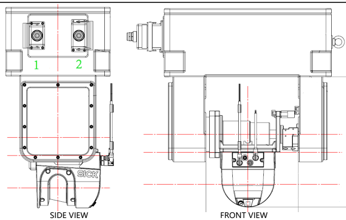
LEFT PORTAL BEAM LEADING POSITION UNIT
